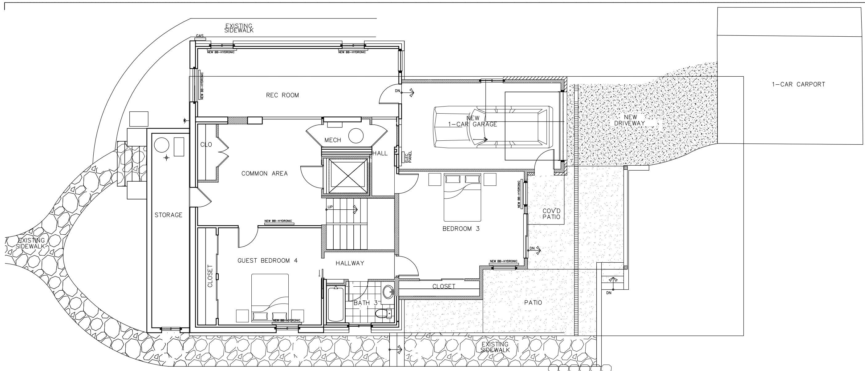
PROPOSED LOWER LEVEL PLAN
