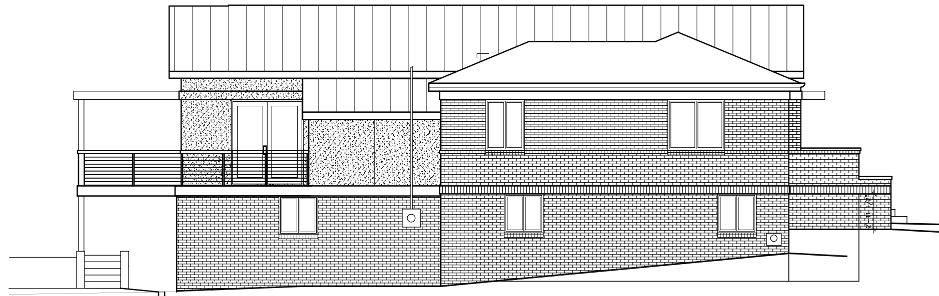
PROPOSED LEFT ELEVATION— NORTH
